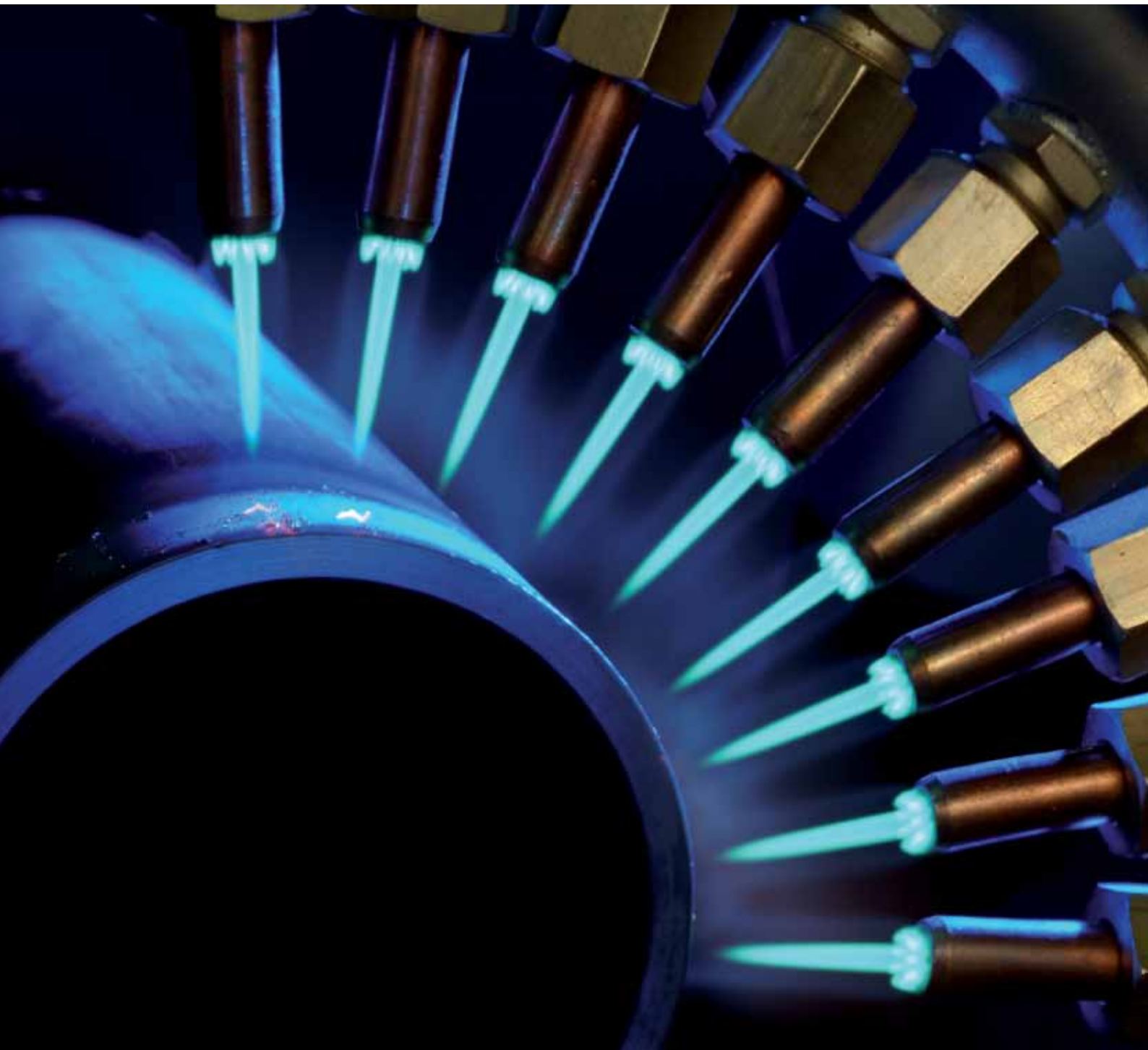
Pipe preheating using air-acetylene LINDOFLAMM® burners
