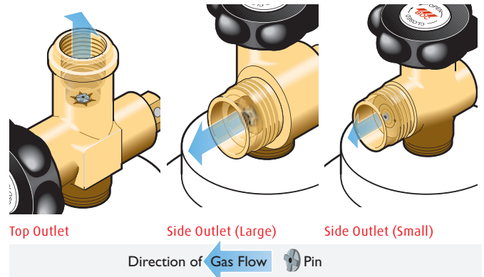
Examining the cylinder valve outlet
